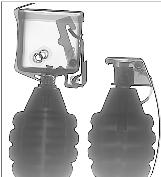
140 kV – 0.3 mA higher contrast
